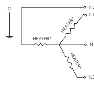
THREE-PHASE WYE CIRCUIT
