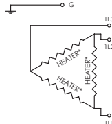
THREE-PHASE DELTA CIRCUIT
