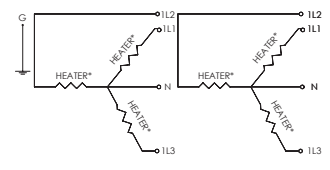
TWO THREE-PHASE WYE CIRCUITS
