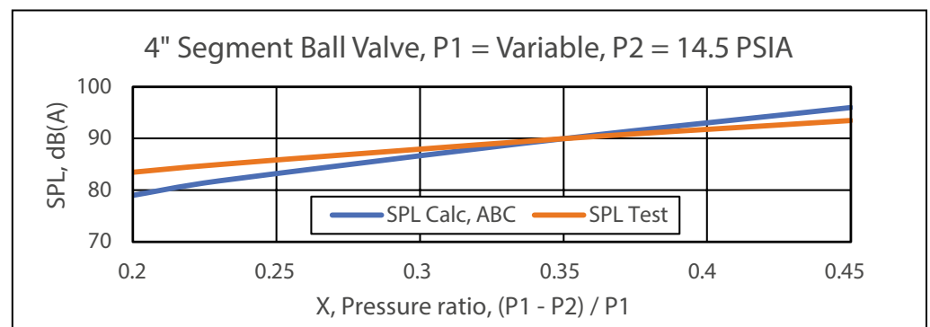
Figure 1. Comparison with an actual blowdown noise test.
